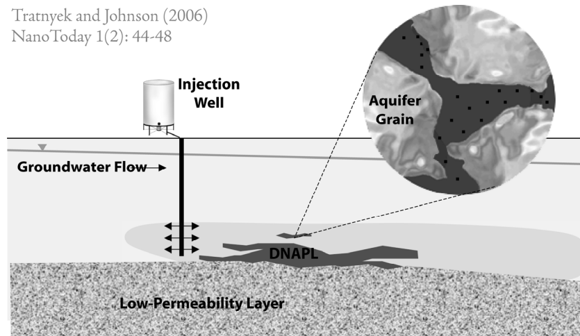
Figure 8. Schematic of two methods of groundwater remediation using nanoiron (Tratnyek, 2006)
