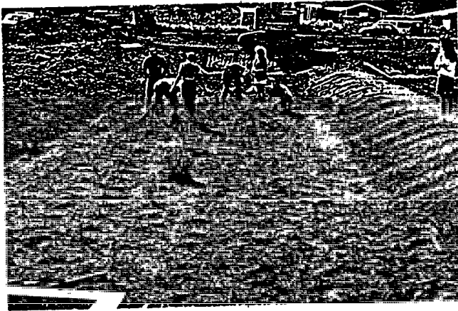
13. After flooding the wetland to settle the substrate, the wetland should be drained for planting.
