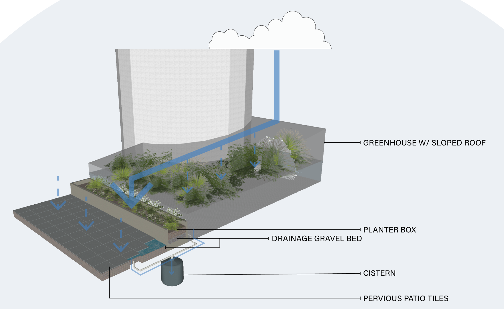
GREENHOUSE + GREYWATER SYSTEM
