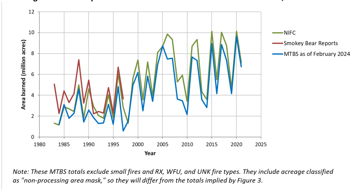
Figure TD-2. Comparison of Wildfire Extent from Three Data Sources, 1983–2021
