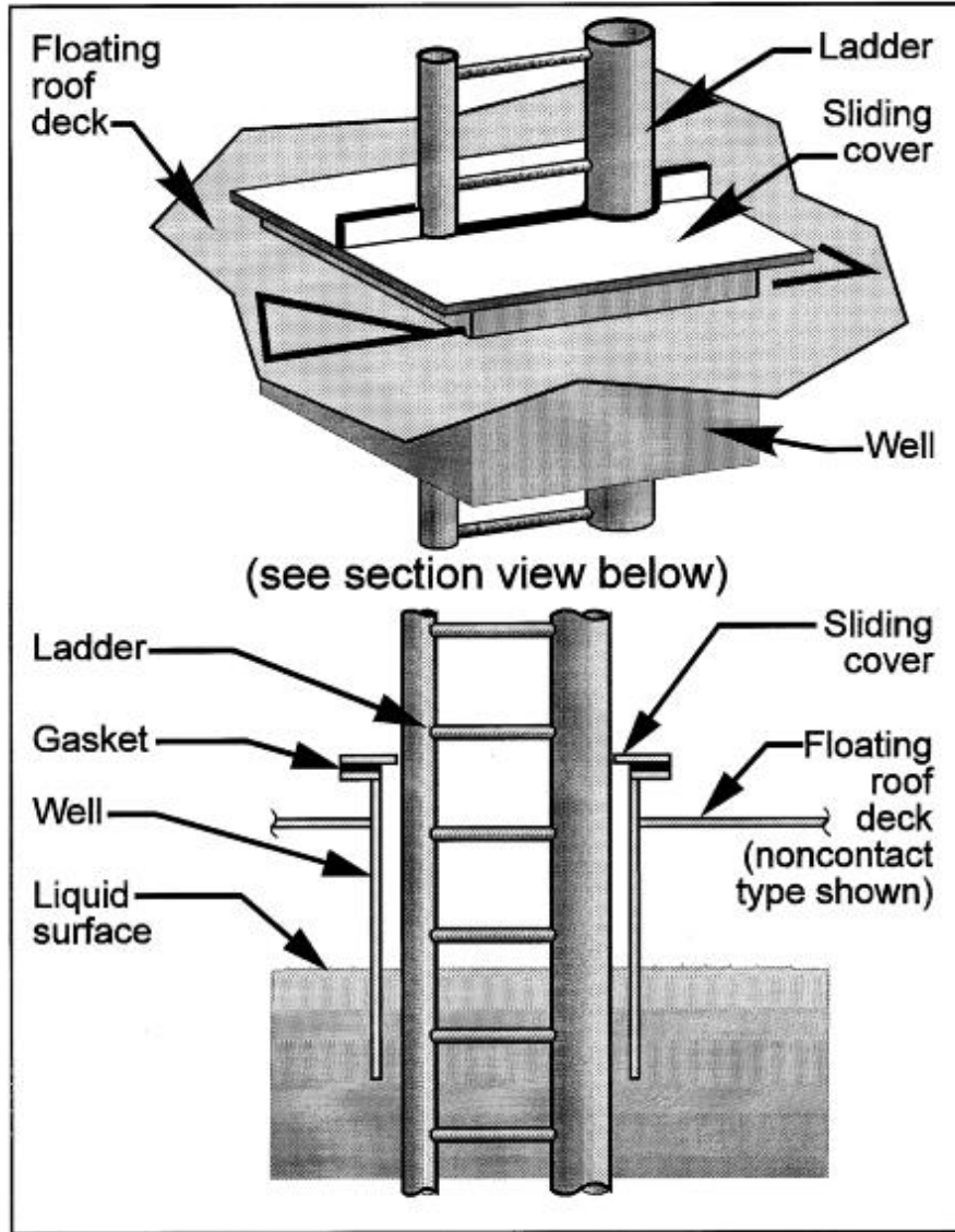
Figure 7.1-12. Ladder well. 20
